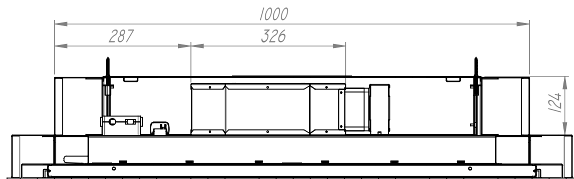
INTERNAL VIEW
