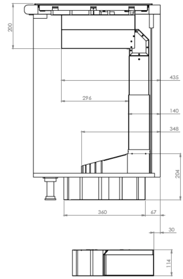
Cut-out dimensions for hob: 750 x 490mm
